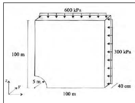
Figure 1 , tunnels dimension and pressure load
