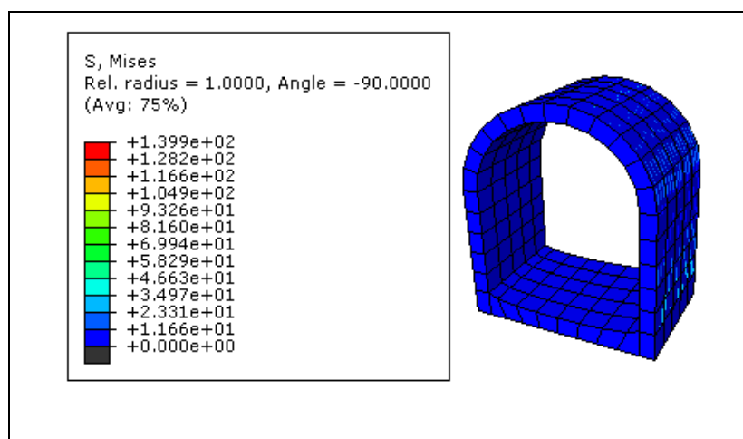
Figure 16 Effect of 60 KN pressure load on the von misses stress
