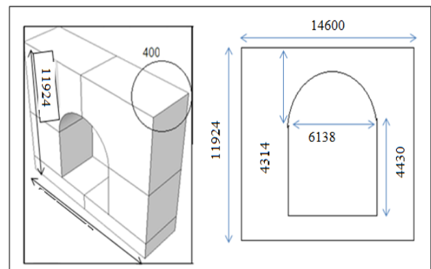
figure 8 soil dimation behind tunnel structure Table1 soil and Tunnel dimension
