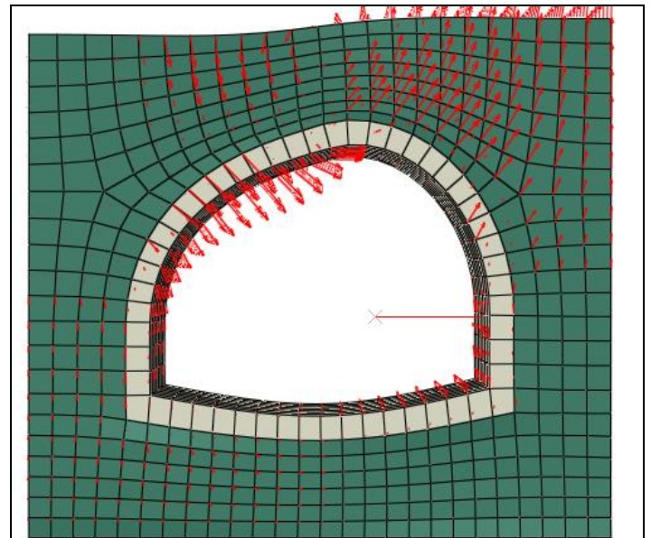
Figure 12 lateral displacement for tunnel and lining
