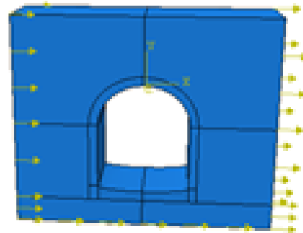
Figure 6 . earth quake load in the soil layer
