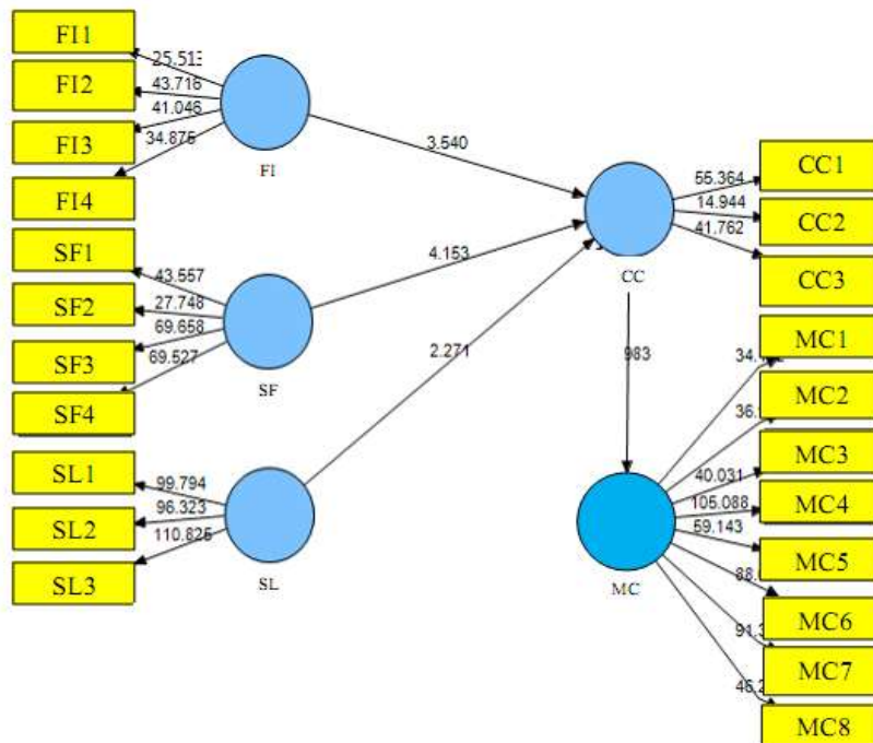
Figure 2.4. Structural research model with significant coefficients
