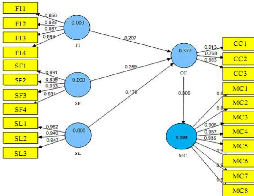
Fig. 4.1. Structural model of research along with factor load factors
